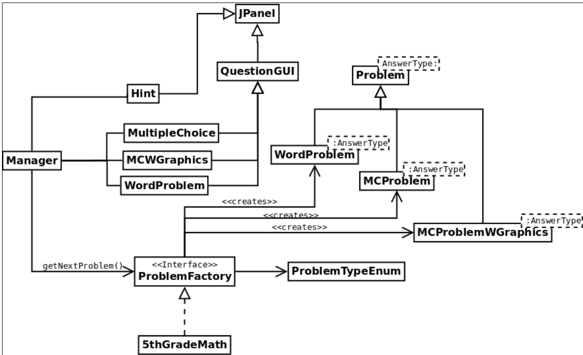
Figure 1: Revised UML
