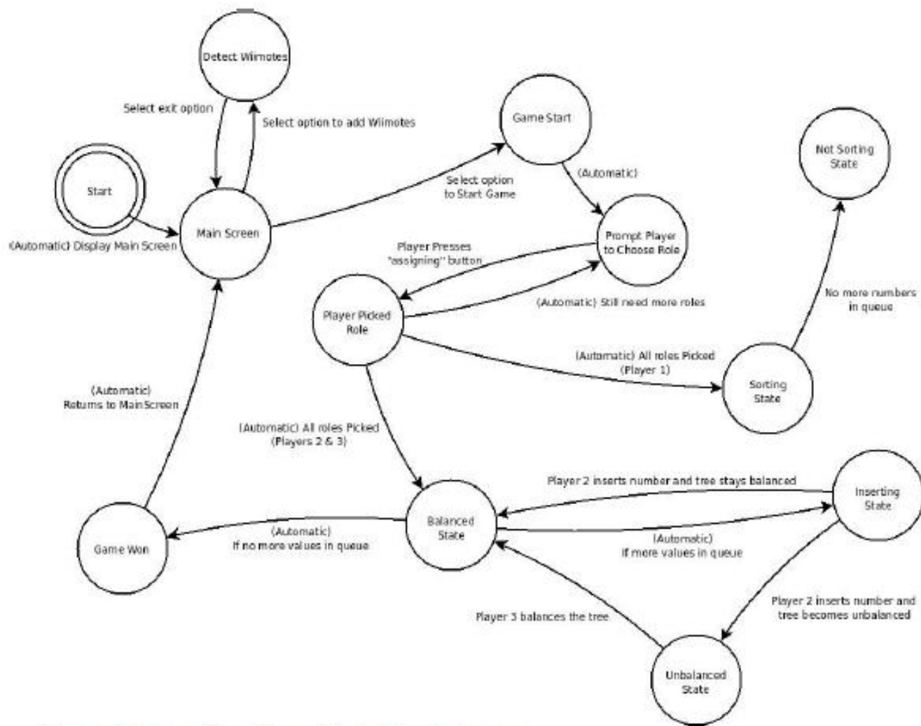
Figure 4: Binary Tree Game Finite State Diagram
