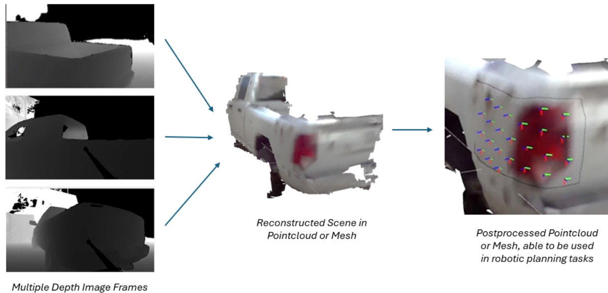
Figure 1: Example pipeline
